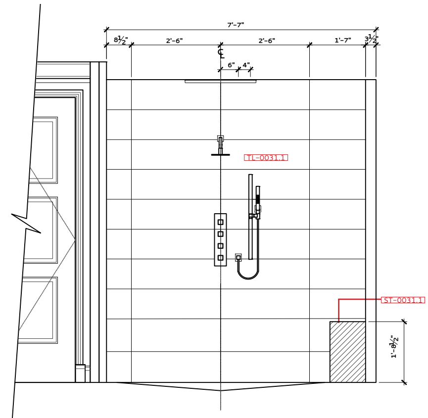
MASTER BATHROOM SHOWER 033 – ELEVATION D
