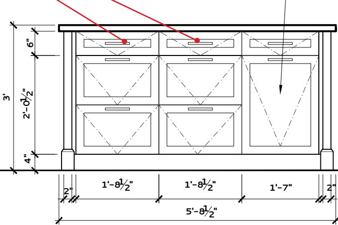
MASTER CLOSET 030 – ISLAND ELEVATION J
