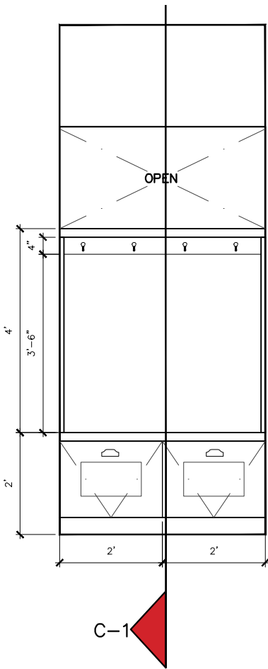
MUDROOM 009B - ELEVATION C
