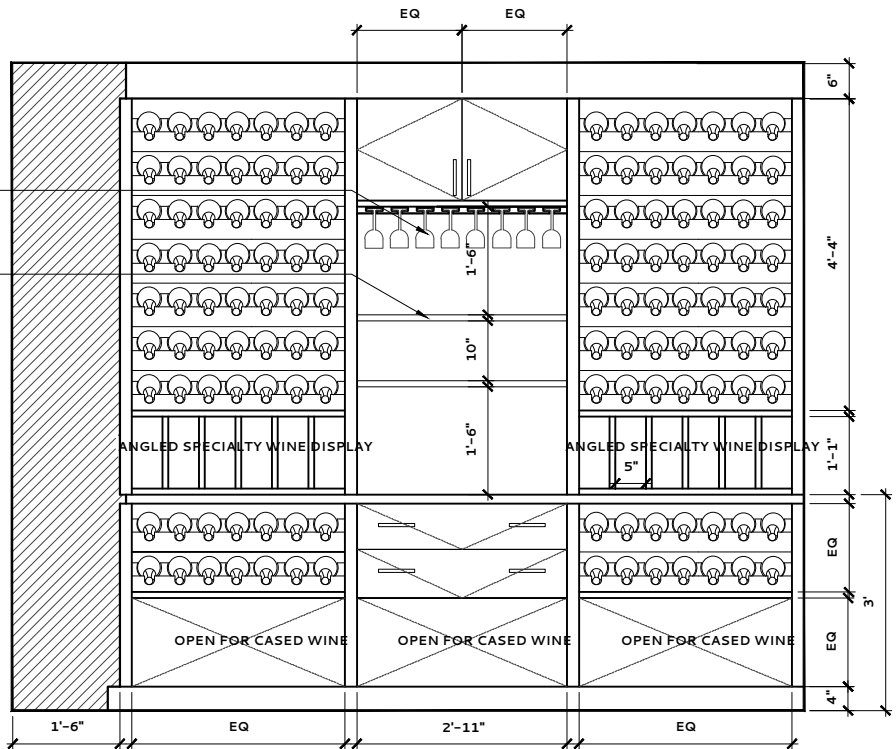
WINE CELLAR 037 - ELEVATION C
