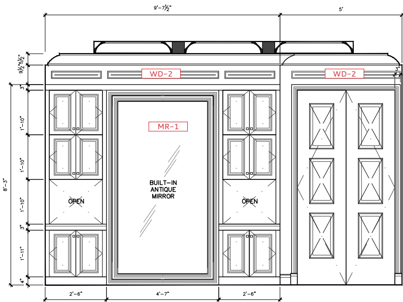
LIBRARY 006 – ELEVATION C
