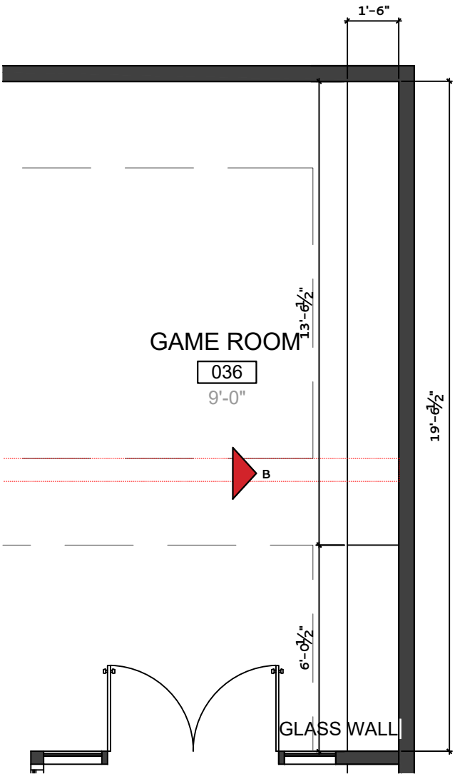
GAME ROOM 036 – FLOOR PLAN
