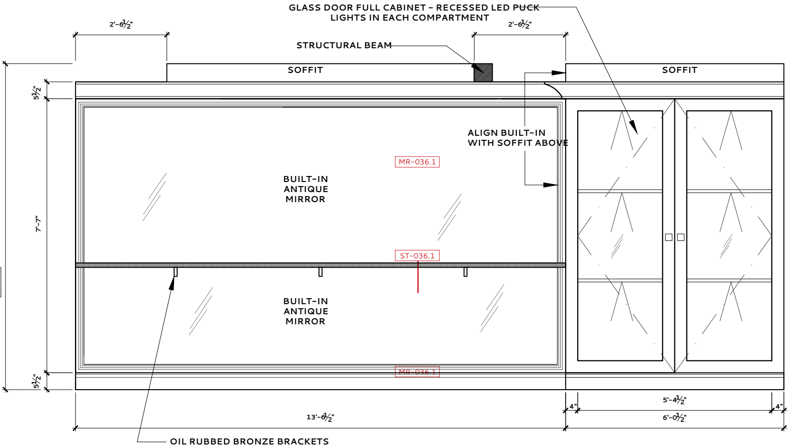
GAME ROOM 036 – FLOOR PLAN
