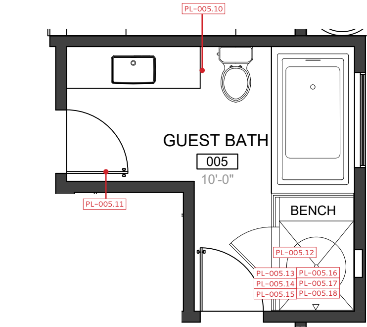
GUEST BATH 005 – FLOOR PLAN
