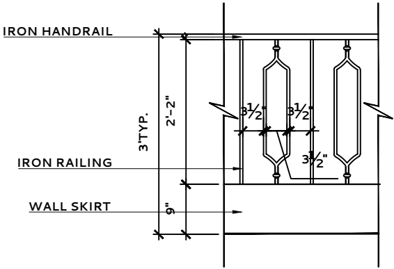
STAIRS 002 – RAIL ELEVATION
