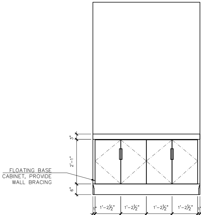
HALL 020 - ELEVATION D
