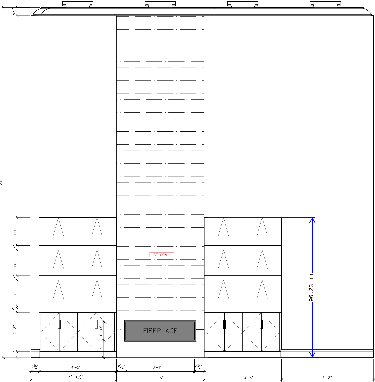
GREAT ROOM 008 – ELEVATION B
