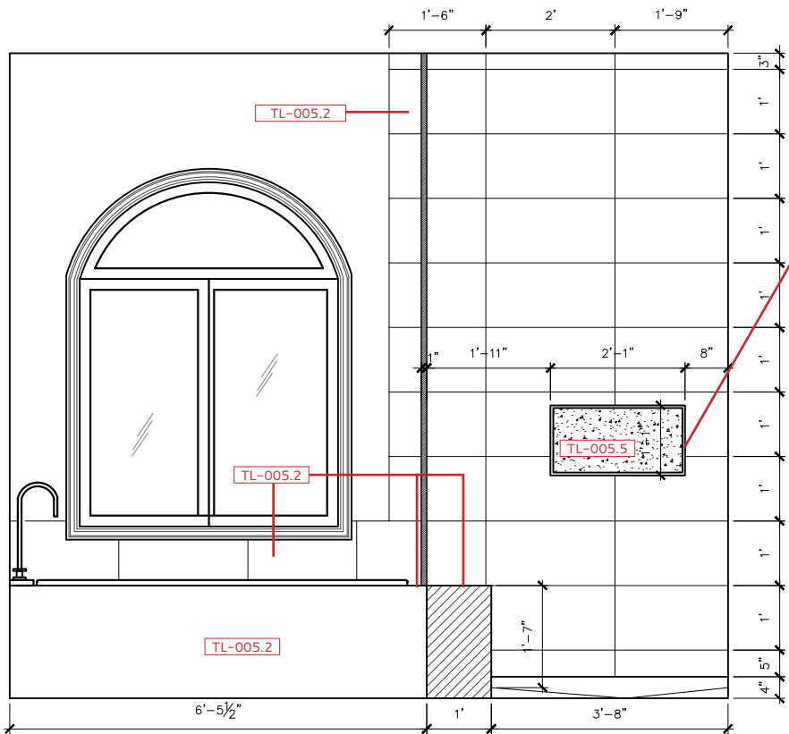
GUEST BATH 005 - ELEVATION B
