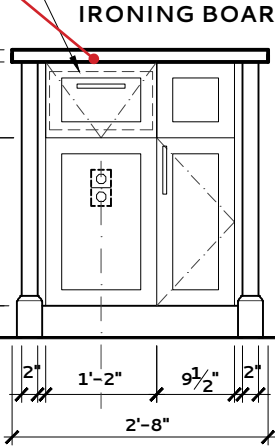
MASTER CLOSET 030 – ISLAND ELEVATION K
