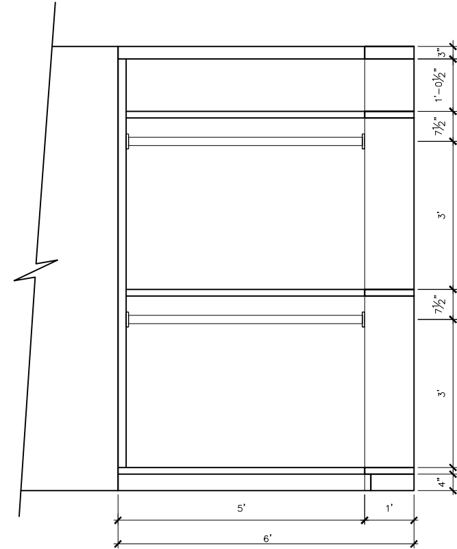
MASTER CLOSET 030 – ELEVATION E
