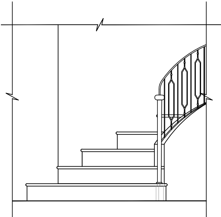
STAIRS 002 – ELEVATION
