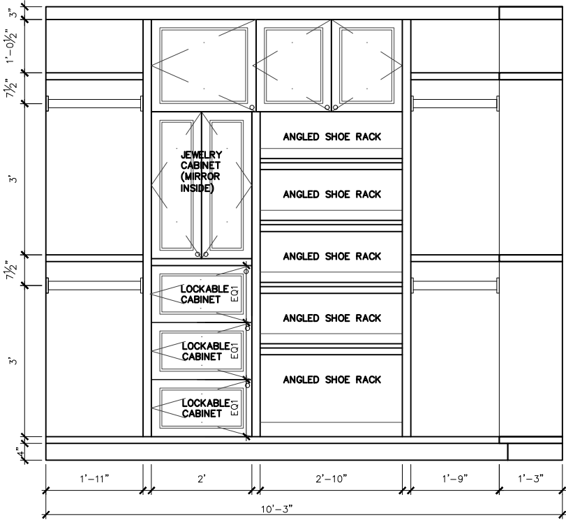
MASTER CLOSET 030 – ELEVATION B
