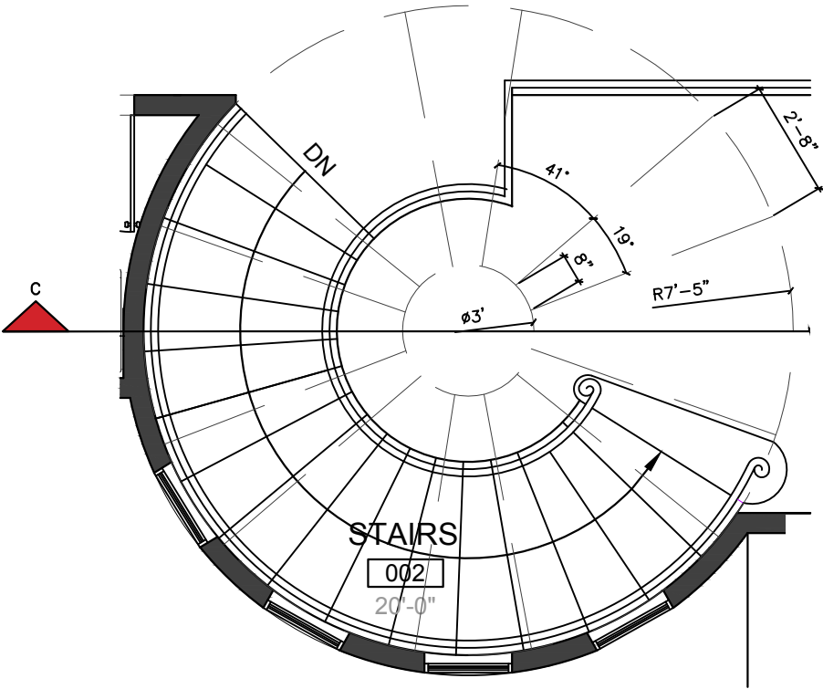
STAIRS 002 – REFLECTIVE CEILING PLAN
