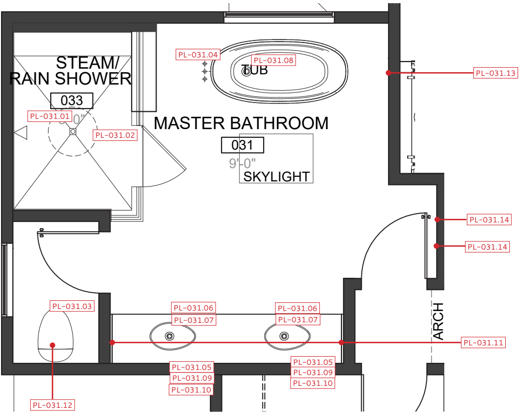
MASTER BATHROOM 031 – FLOOR PLAN
