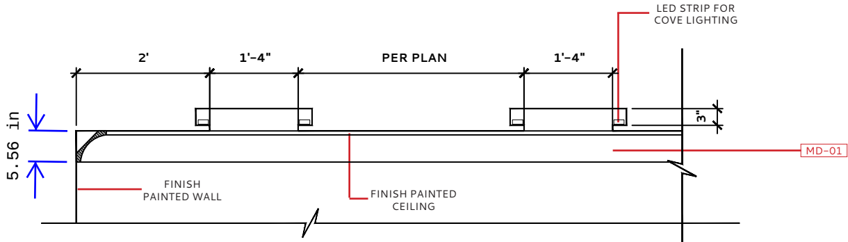
GREAT ROOM 008 – SECTION DETAIL D
