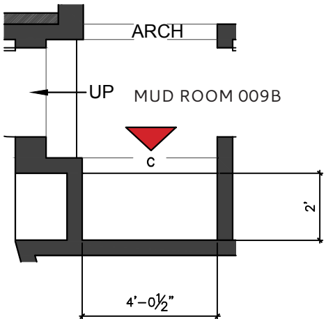
MUD ROOM 009B - FLOOR PLAN
