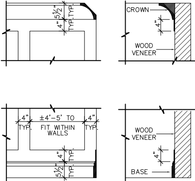
PANELING DETAILS
