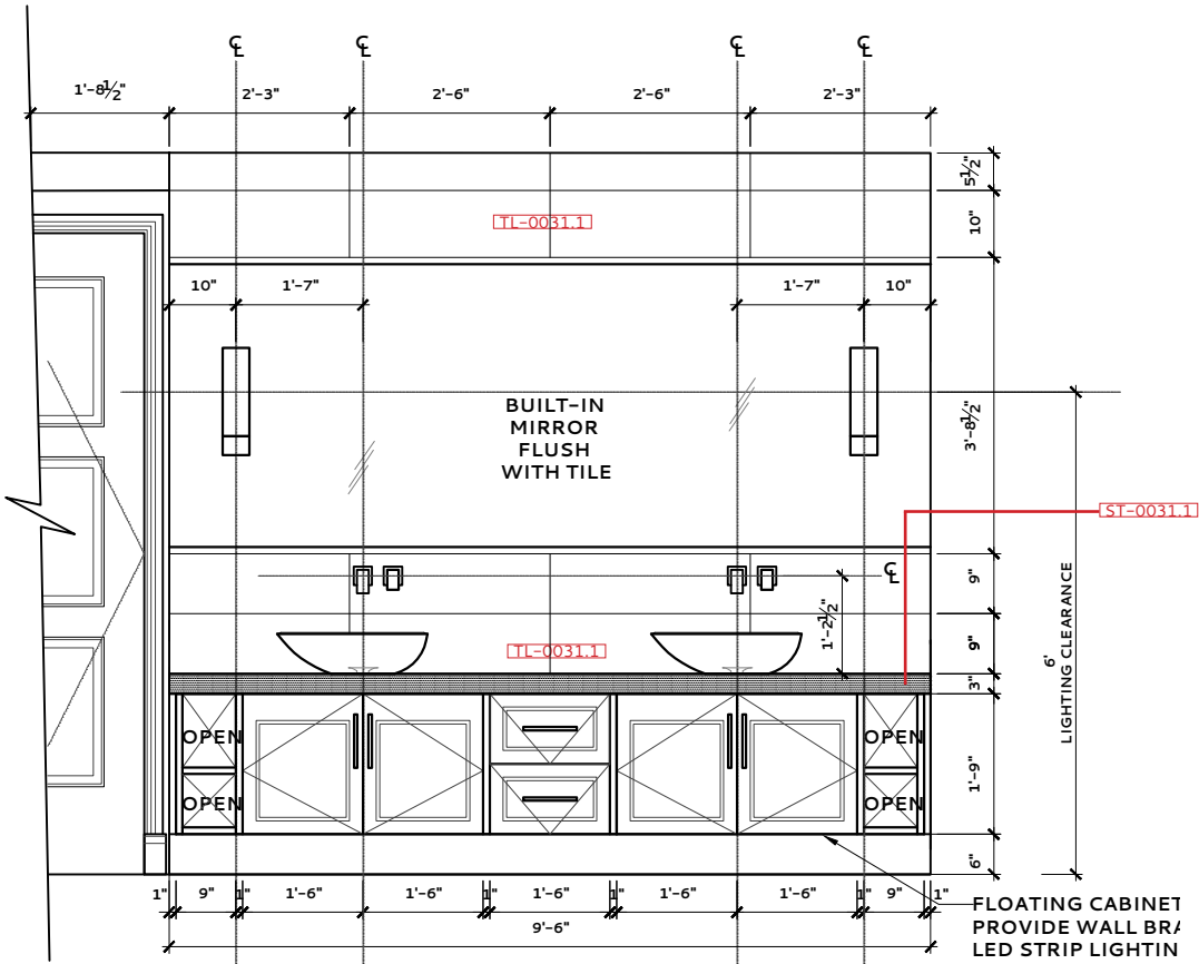
MASTER BATHROOM 031 - ELEVATION C
