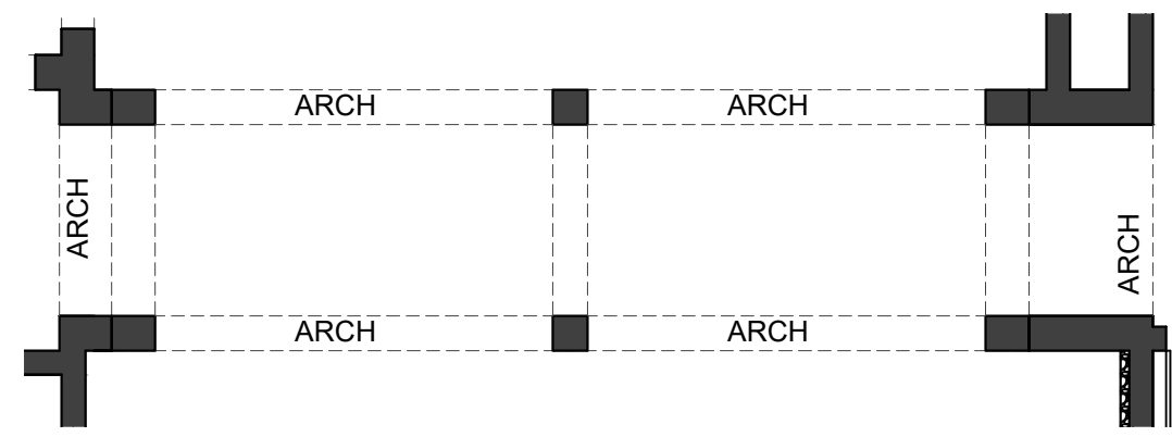
ENTRY 001 - HALL 009 - COLUMNS PLAN SCALE: 1/4" = 1'-0"
