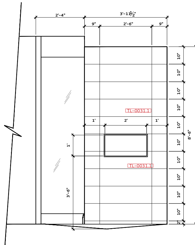
MASTER BATHROOM SHOWER 033 – ELEVATION C
