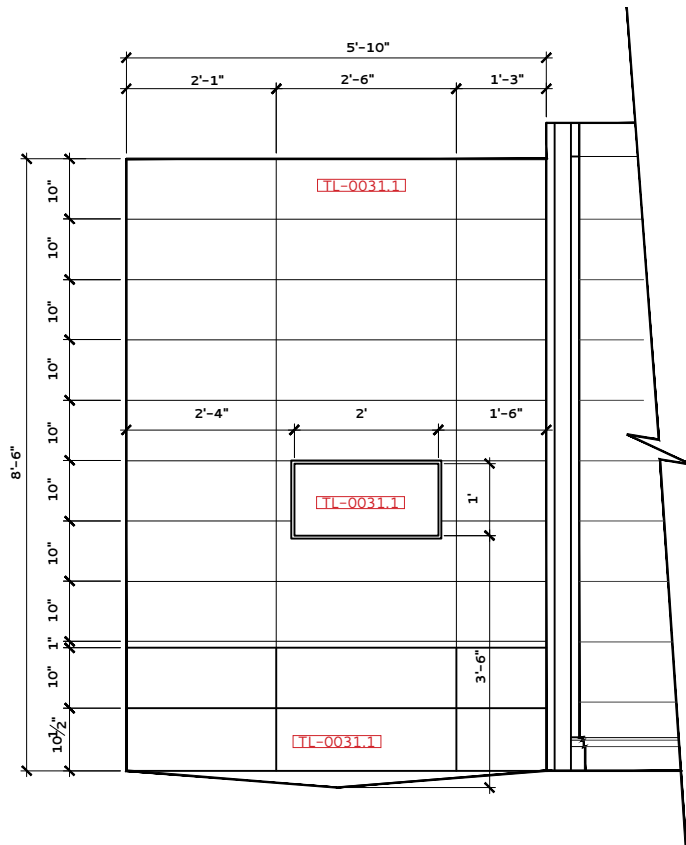
MASTER BATHROOM SHOWER 033 – ELEVATION A
