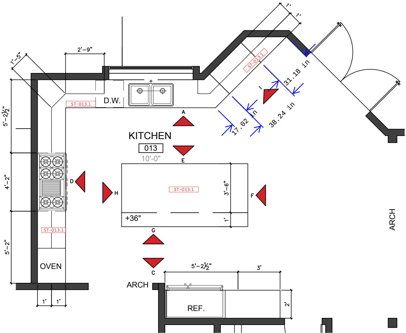
KITCHEN 013 - FLOOR PLAN
