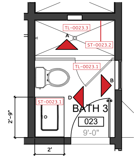
BATH 3 023 - FLOOR PLAN
