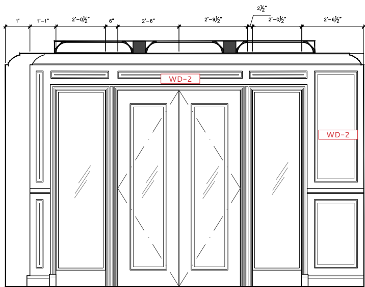
LIBRARY 006 - ELEVATION A
