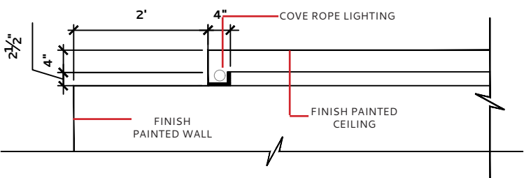
THEATER 040 - SECTION DETAIL F
