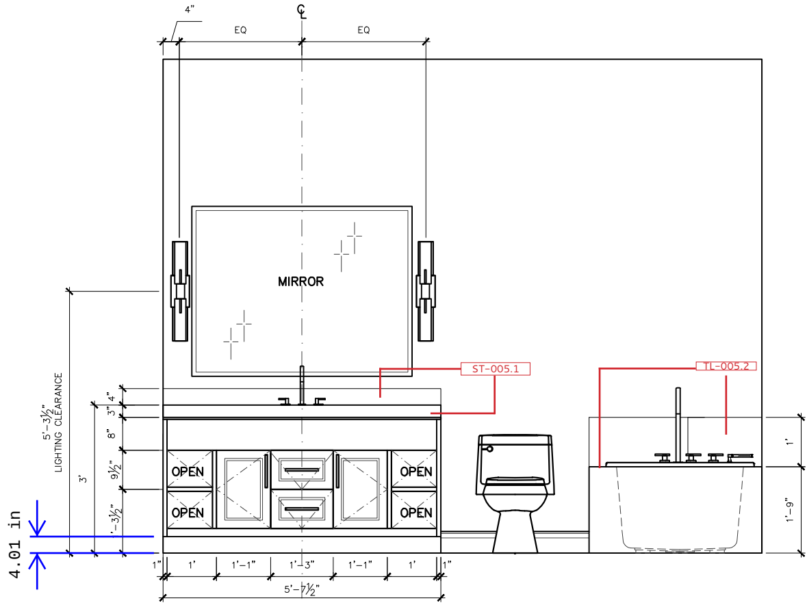
GUEST BATH 005 - ELEVATION A
