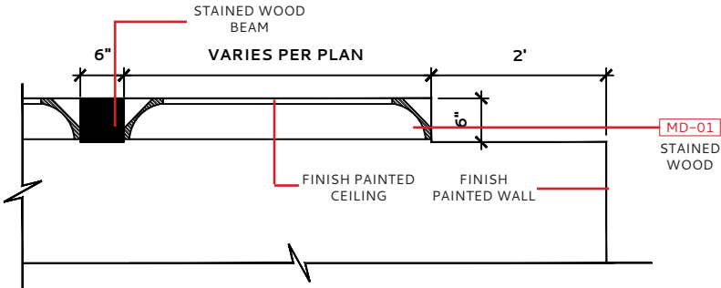
LIBRARY 006 – SECTION DETAIL B
