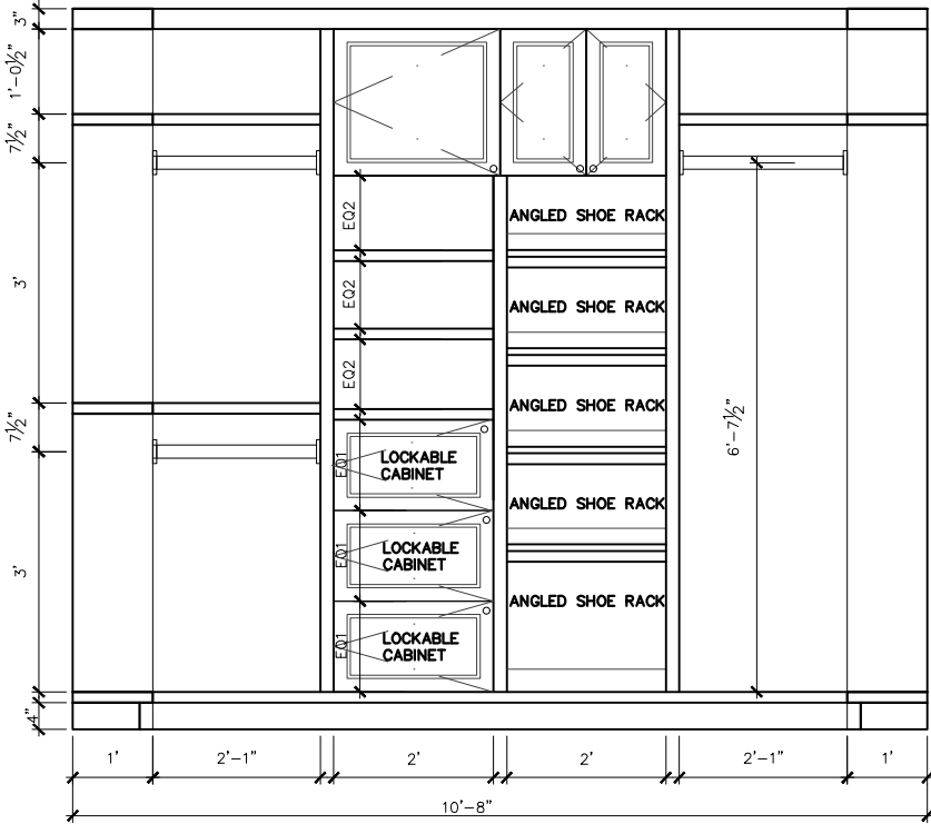
MASTER CLOSET 030 – ELEVATION G
