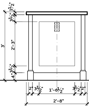
MASTER CLOSET 030 – ISLAND ELEV. I
