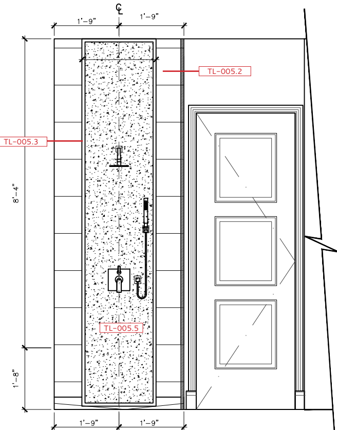
GUEST BATH 005 - ELEVATION C
