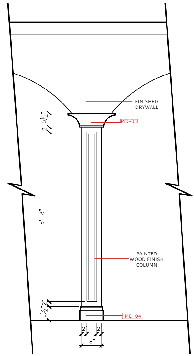
HALL & ENTRY COLUMNS 009 - DETAIL SCALE: 1/2" = 1'-0"
