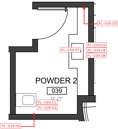
POWDER 039 – FLOOR PLAN
