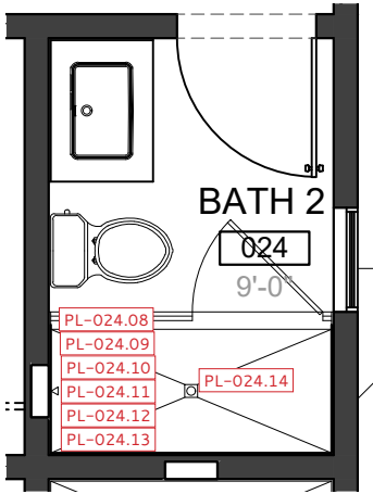
BATH 2 – FLOOR PLAN
