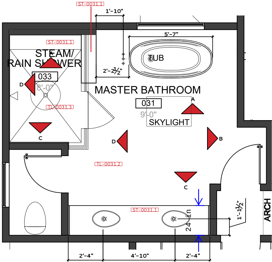
MASTER BATHROOM 031 - FLOOR PLAN
