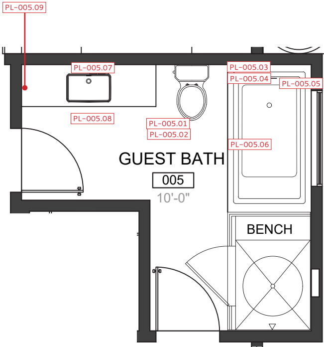
GUEST BATH – FLOOR PLAN
