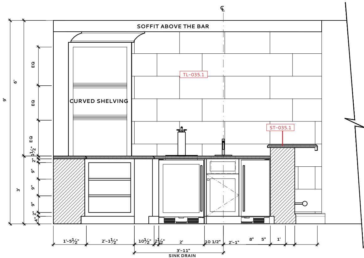
BAR 035 – ELEVATION D
