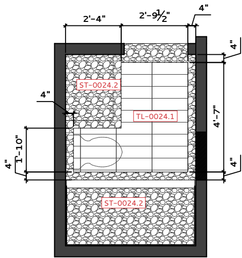
BATH 2 024 - FLOORING DETAIL PLAN
