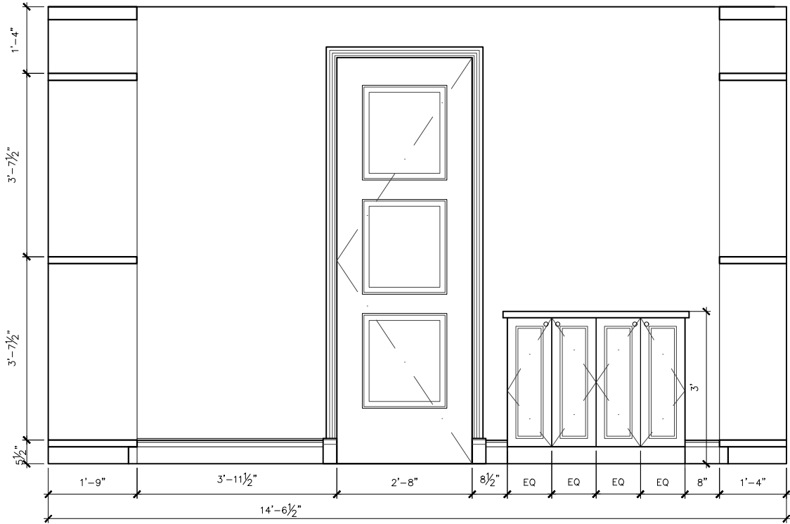
MASTER CLOSET 030 – ELEVATION A
