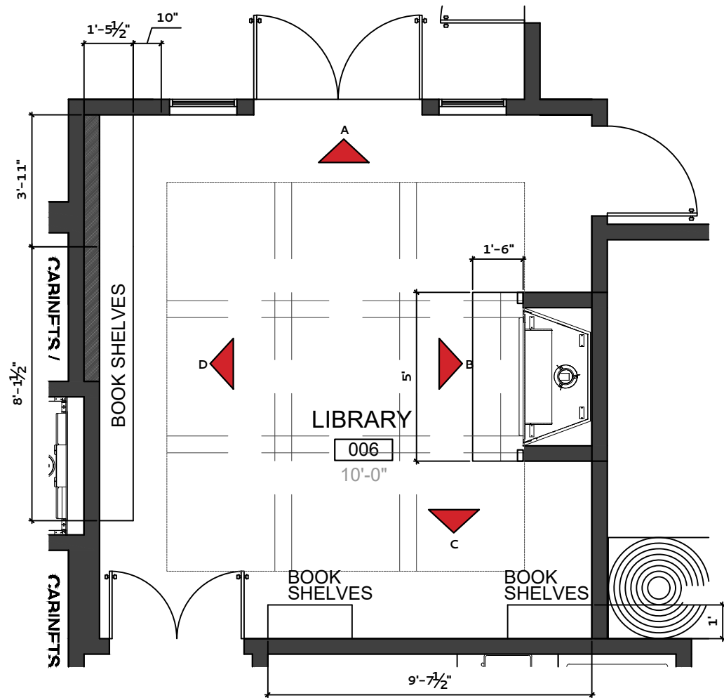
LIBRARY 006 - FLOOR PLAN
