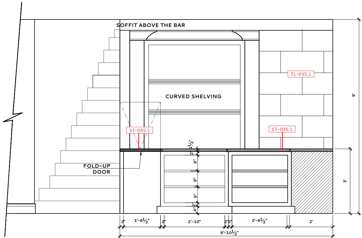
BAR 035 – ELEVATION C
