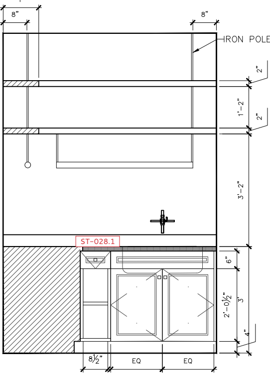
LAUNDRY ROOM 0280 - ELEVATION D
