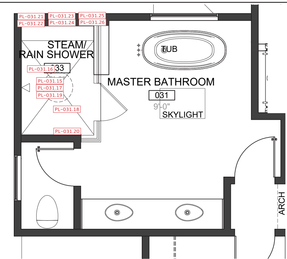
MASTER BATHROOM 031 – FLOOR PLAN
