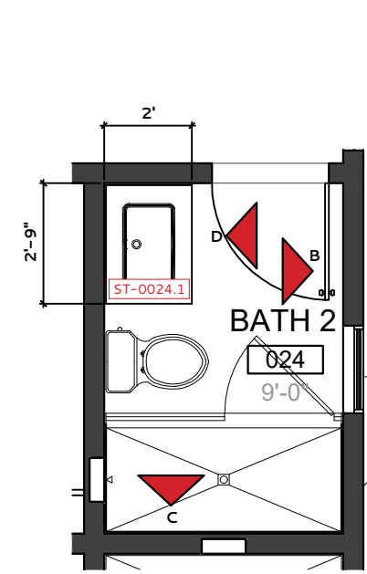
BATH 2 024 - FLOOR PLAN
