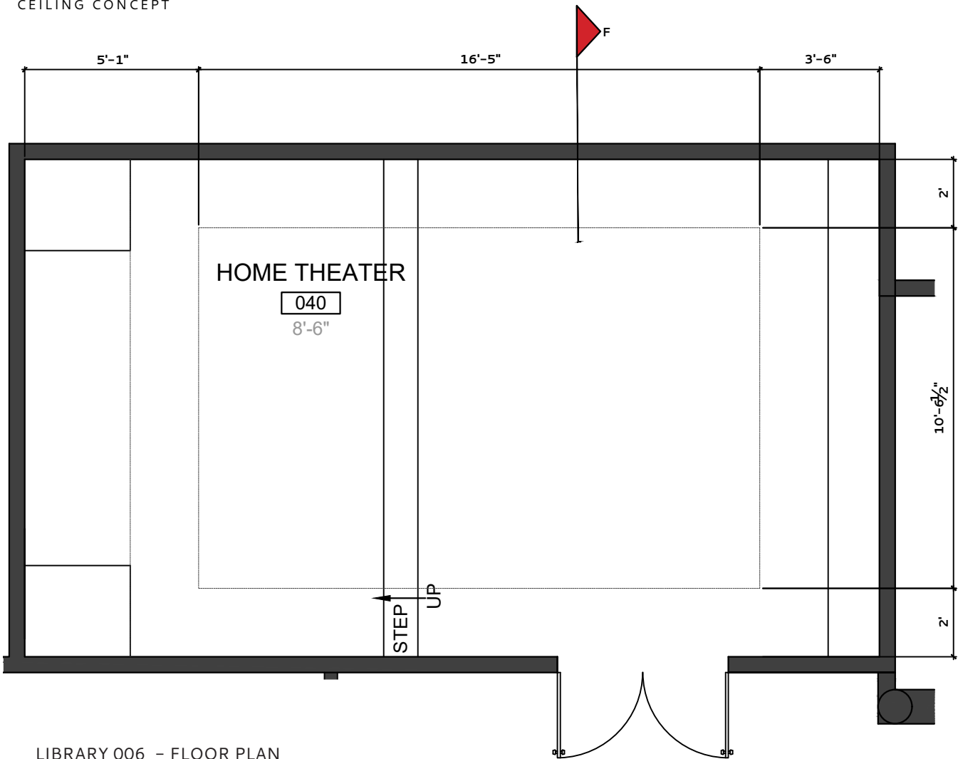
LIBRARY 006 - FLOOR PLAN
