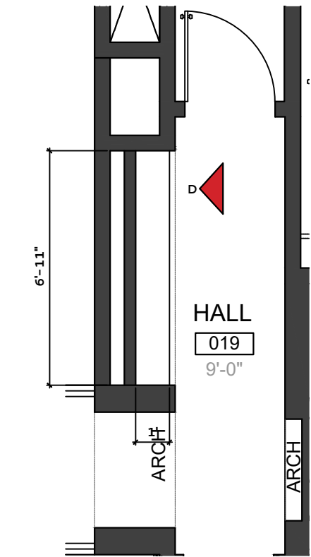
HALL 019 - FLOOR PLAN
