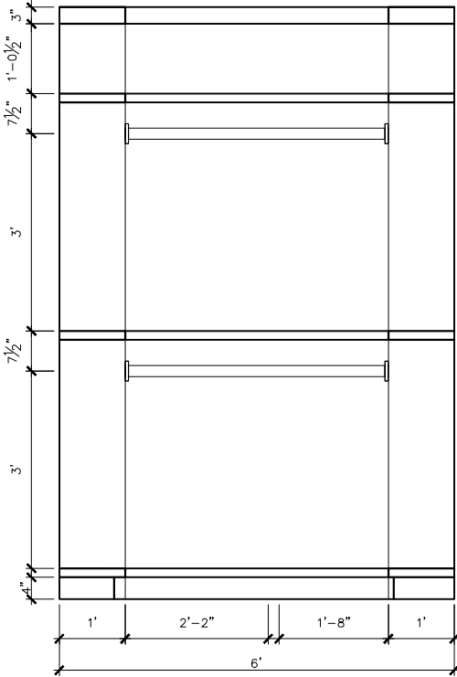
MASTER CLOSET 030 – ELEVATION F
