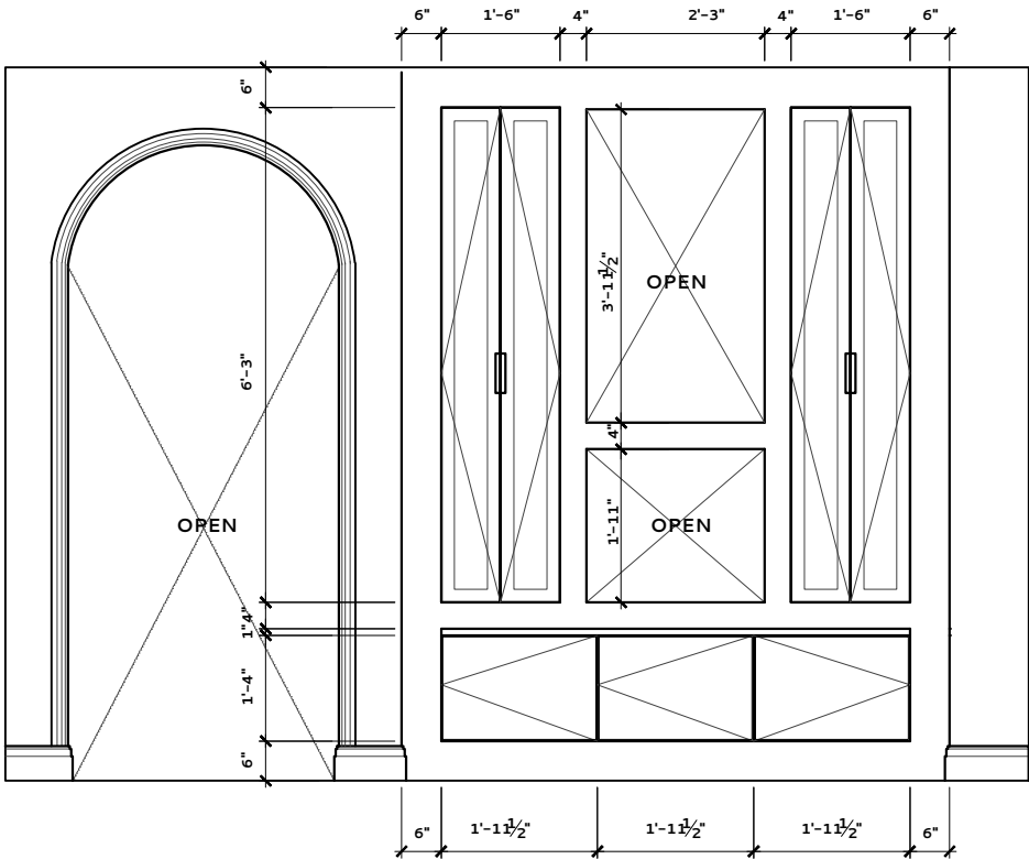
HALL 019 - ELEVATION D
