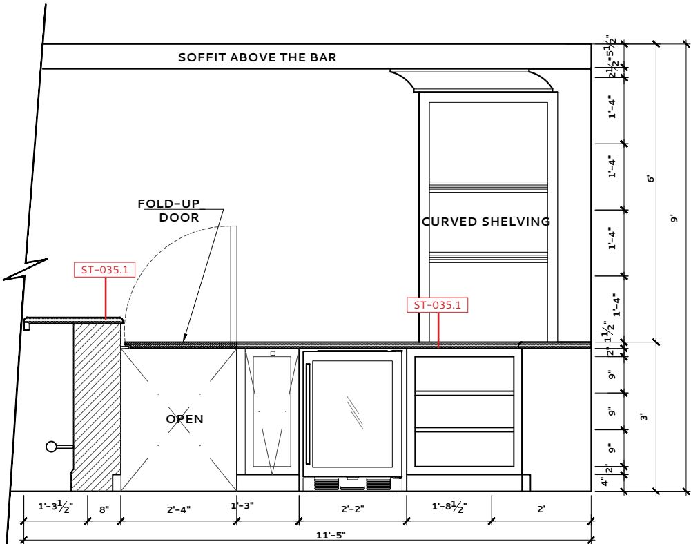
BAR 035 – ELEVATION B
