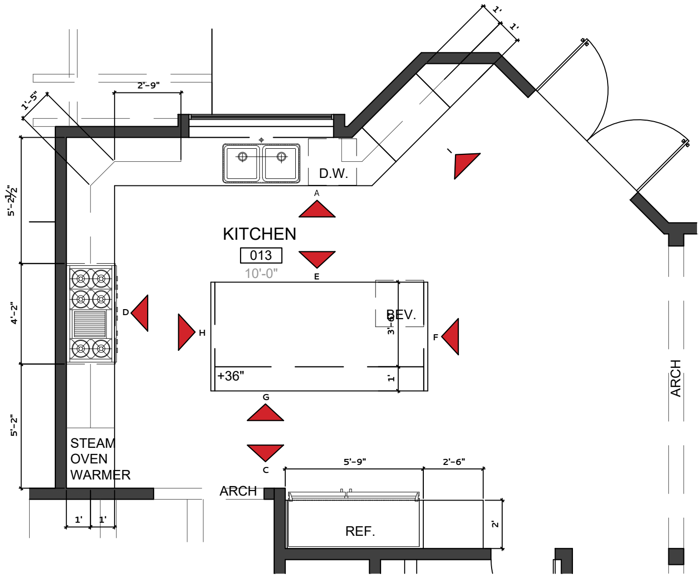
KITCHEN 013 - FLOOR PLAN
