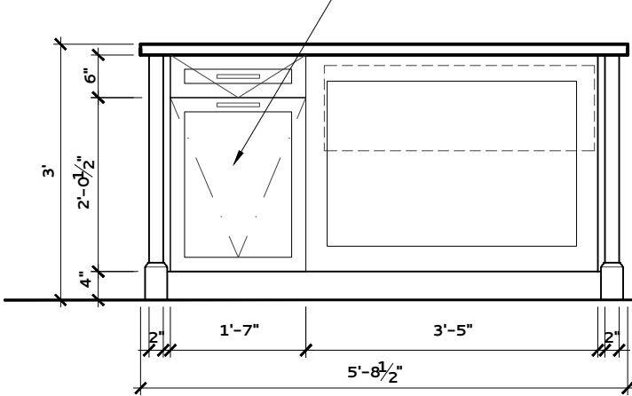
MASTER CLOSET 030 – ISLAND ELEVATION H
