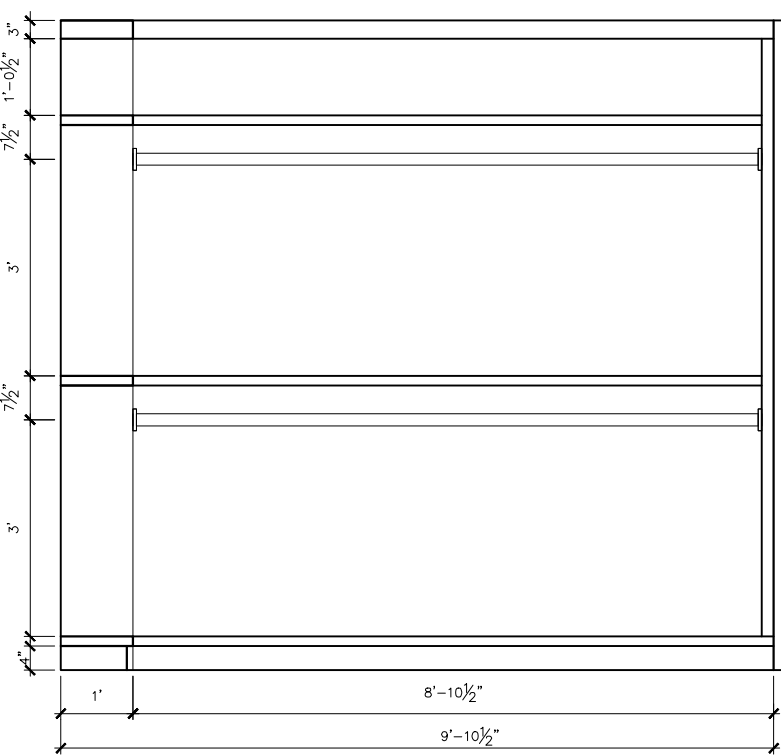
MASTER CLOSET 030 – ELEVATION C
