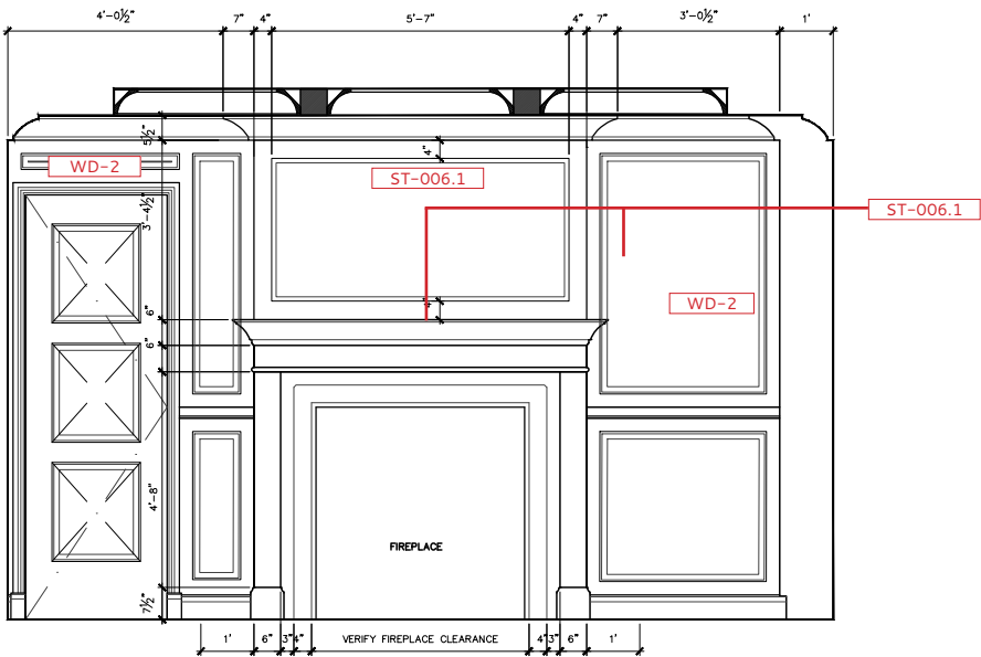
LIBRARY 006 - ELEVATION B
