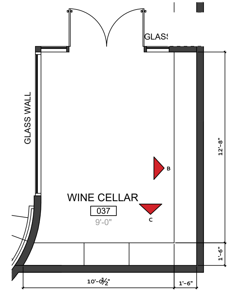
WINE CELLAR 037 - FLOOR PLAN
