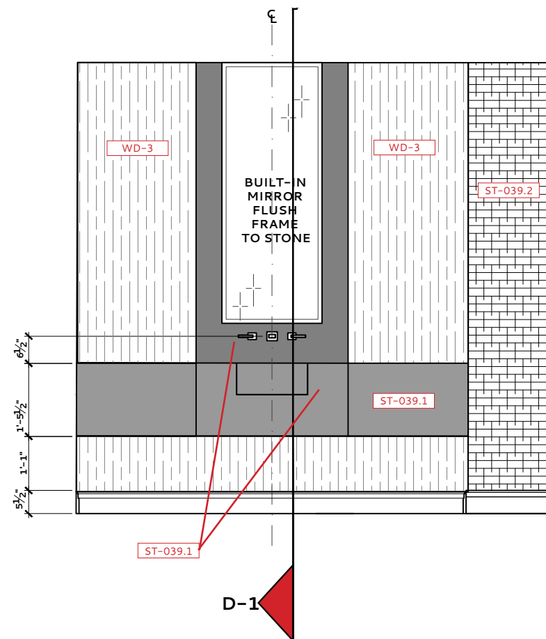
POWDER 2 039 – ELEVATION B
