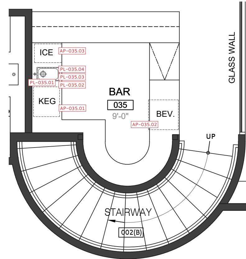
BAR - FLOOR PLAN
