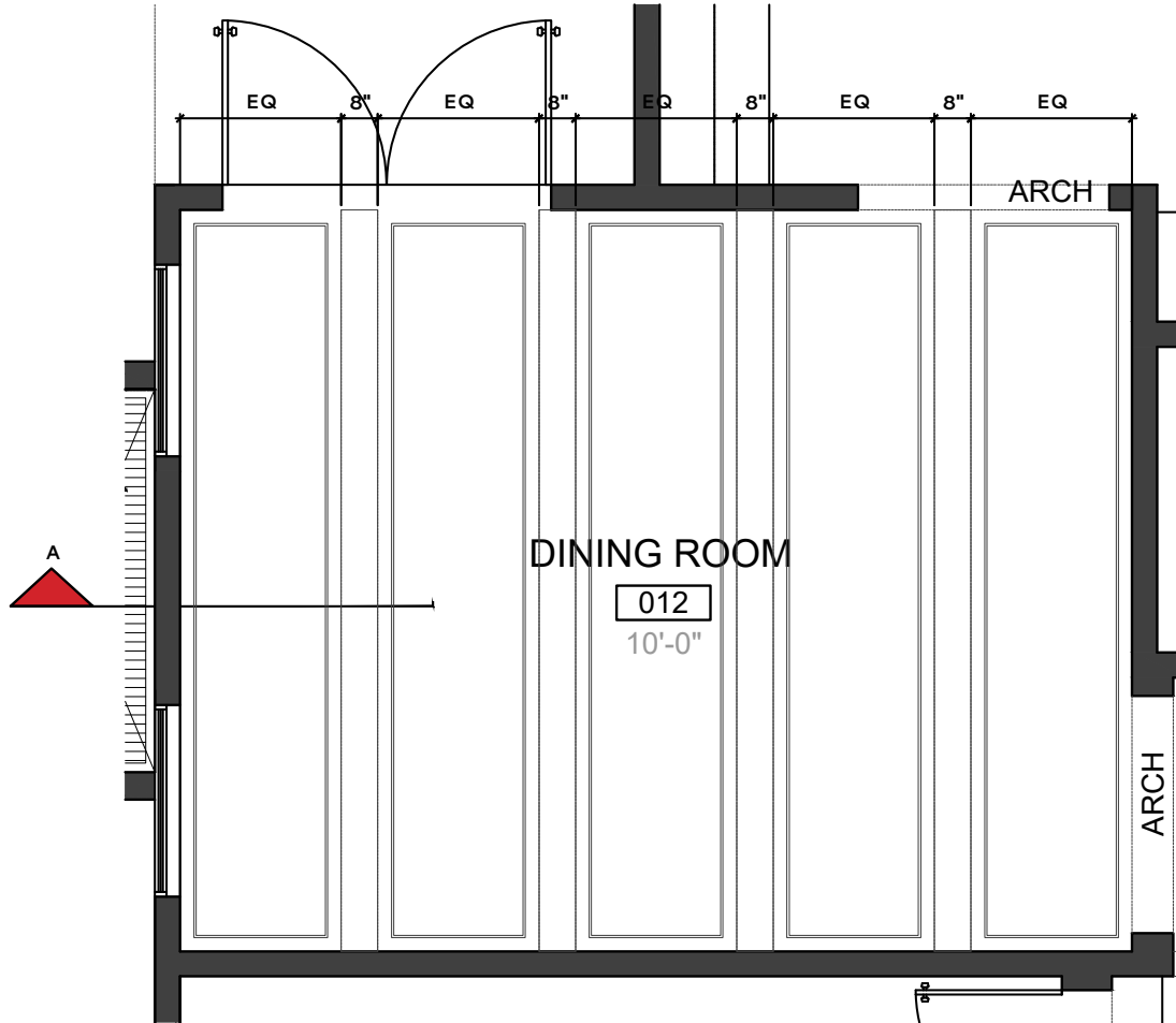
CEILING CONCEPT
