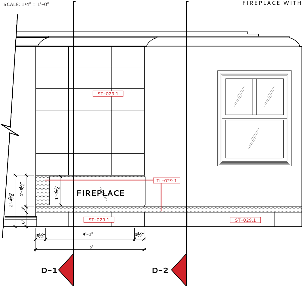
MASTER BEDROOM 029 - FIREPLACE ELEVATION D
