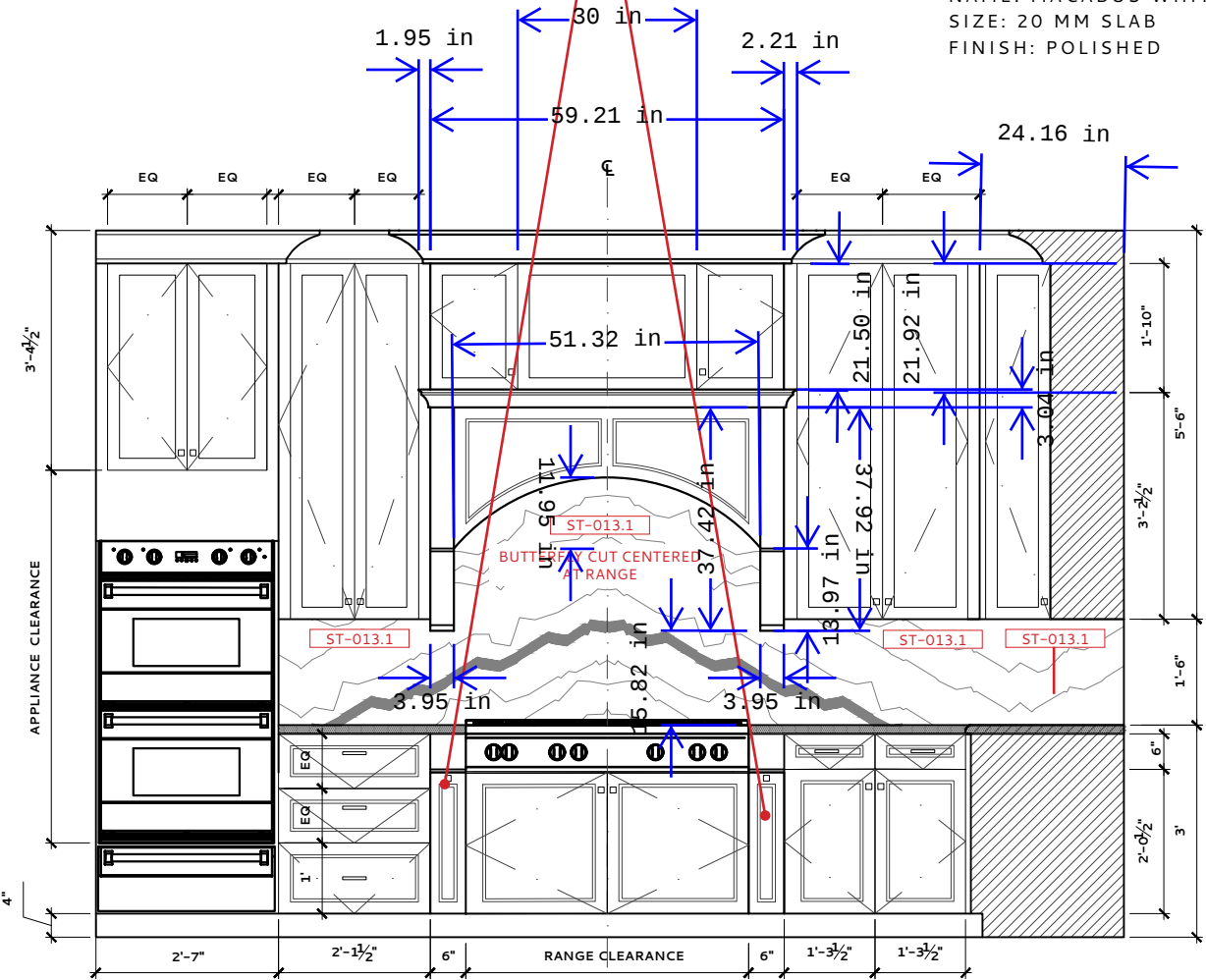
KITCHEN 013 - ELEVATION D
