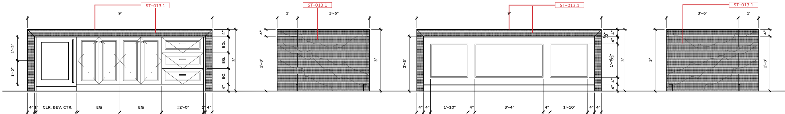
KITCHEN 013 - ISLAND ELEVATION E
