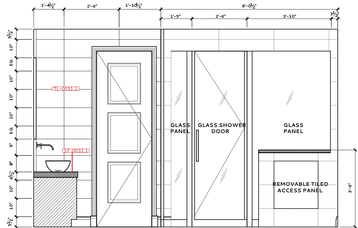
MASTER BATHROOM 031 - ELEVATION D
