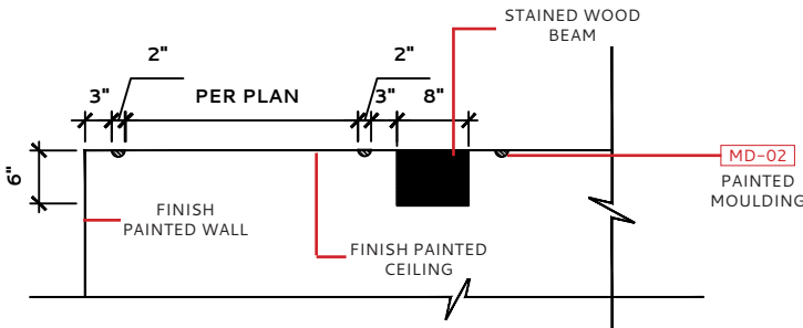
DINING ROOM 012 – SECTION DETAIL A
