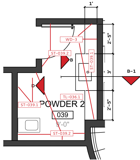
POWDER 2 039 – FLOOR PLAN
