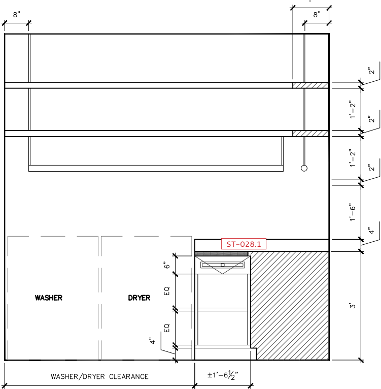
LAUNDRY ROOM 0280 - ELEVATION C
