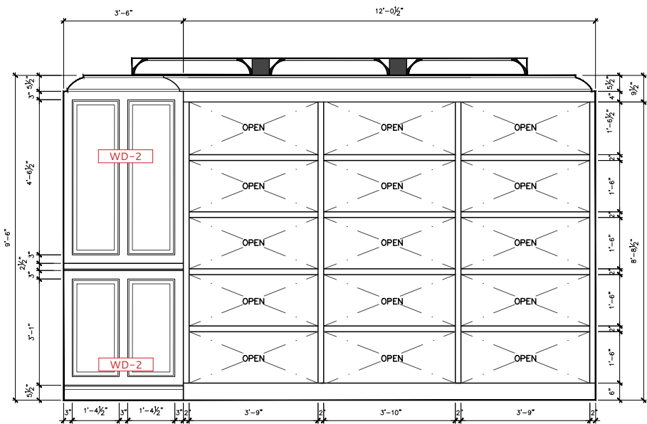
LIBRARY 006 – ELEVATION D
