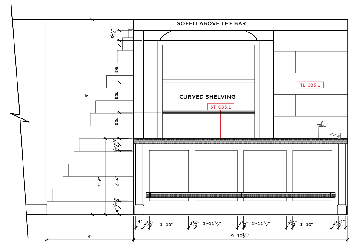
BAR 035 – ELEVATION E
