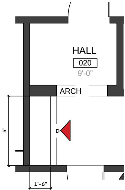
HALL 020 - FLOOR PLAN
