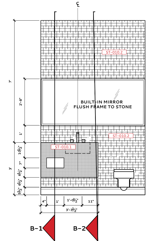
POWDER 010 – ELEVATION B
