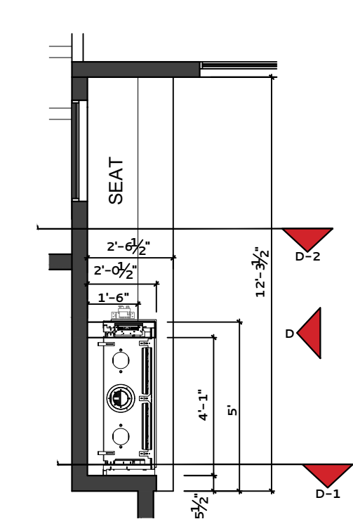
MASTER BEDROOM 029 - FLOOR PLAN
