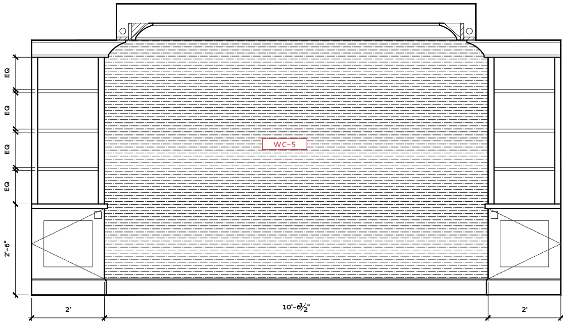
HOME THEATER 040 - ELEVATION D
