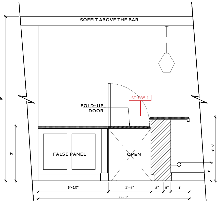
BAR 035 – ELEVATION F
