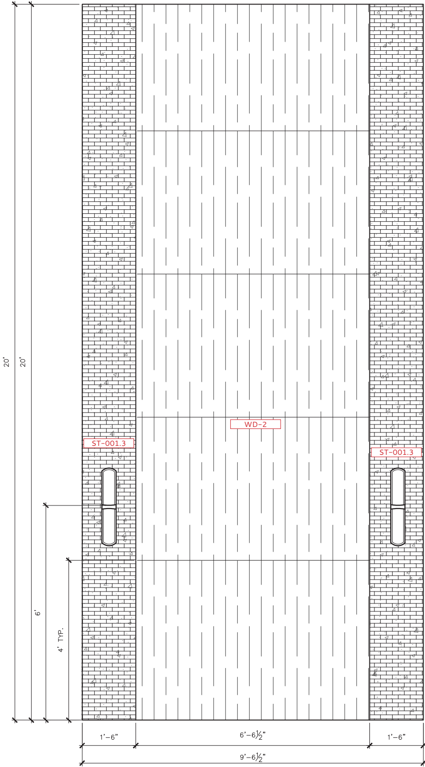
ENTRY 001 – ELEVATION B
