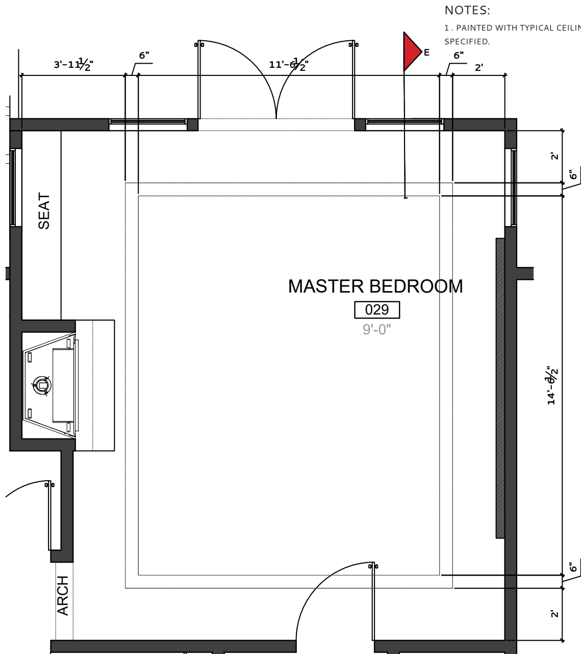
MASTER BEDROOM 029 - FLOOR PLAN
