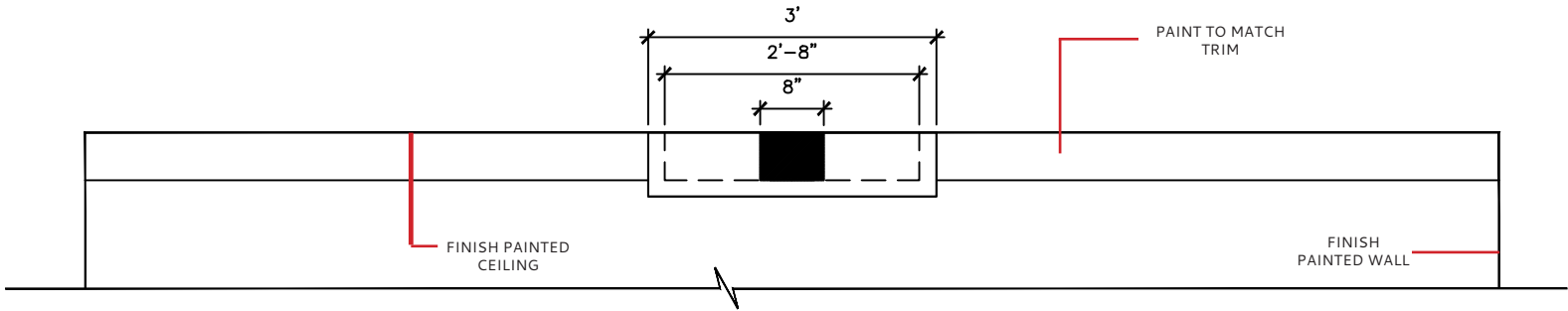
STAIRS 002 – SECTION DETAIL C
