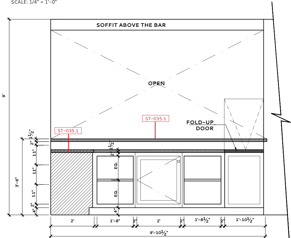
BAR 035 – ELEVATION A
