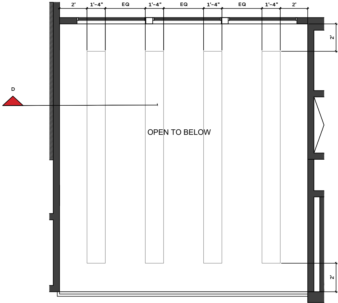
GREAT ROOM 008 – REFLECTIVE CEILING PLAN
