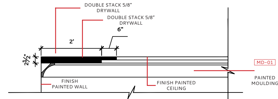
MASTER BEDROOM 029 - SECTION DETAIL E
