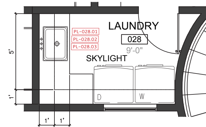
LAUNDRY – FLOOR PLAN
