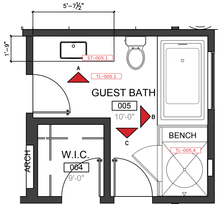
GUEST BATH 005 - FLOOR PLAN
